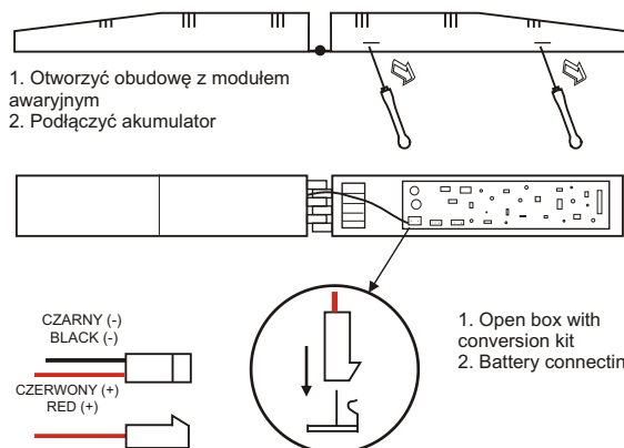
BATTERY CONNECTION
